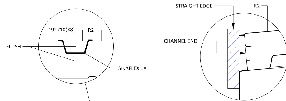
192522 (SEALANT)
