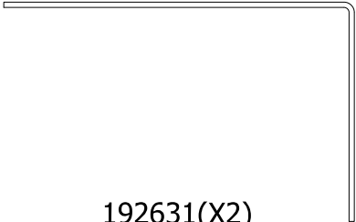
192631(X2) 4" X 2 1/2" X 86 3/8" ANGLE
